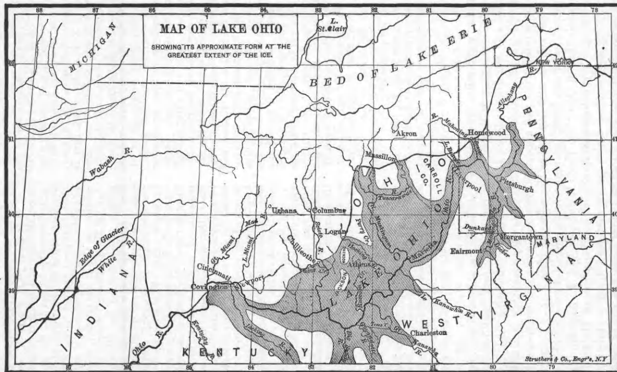
From Wright's Ice Age in North America ; by courtesy of D. Appleton & Co., Publishers.
